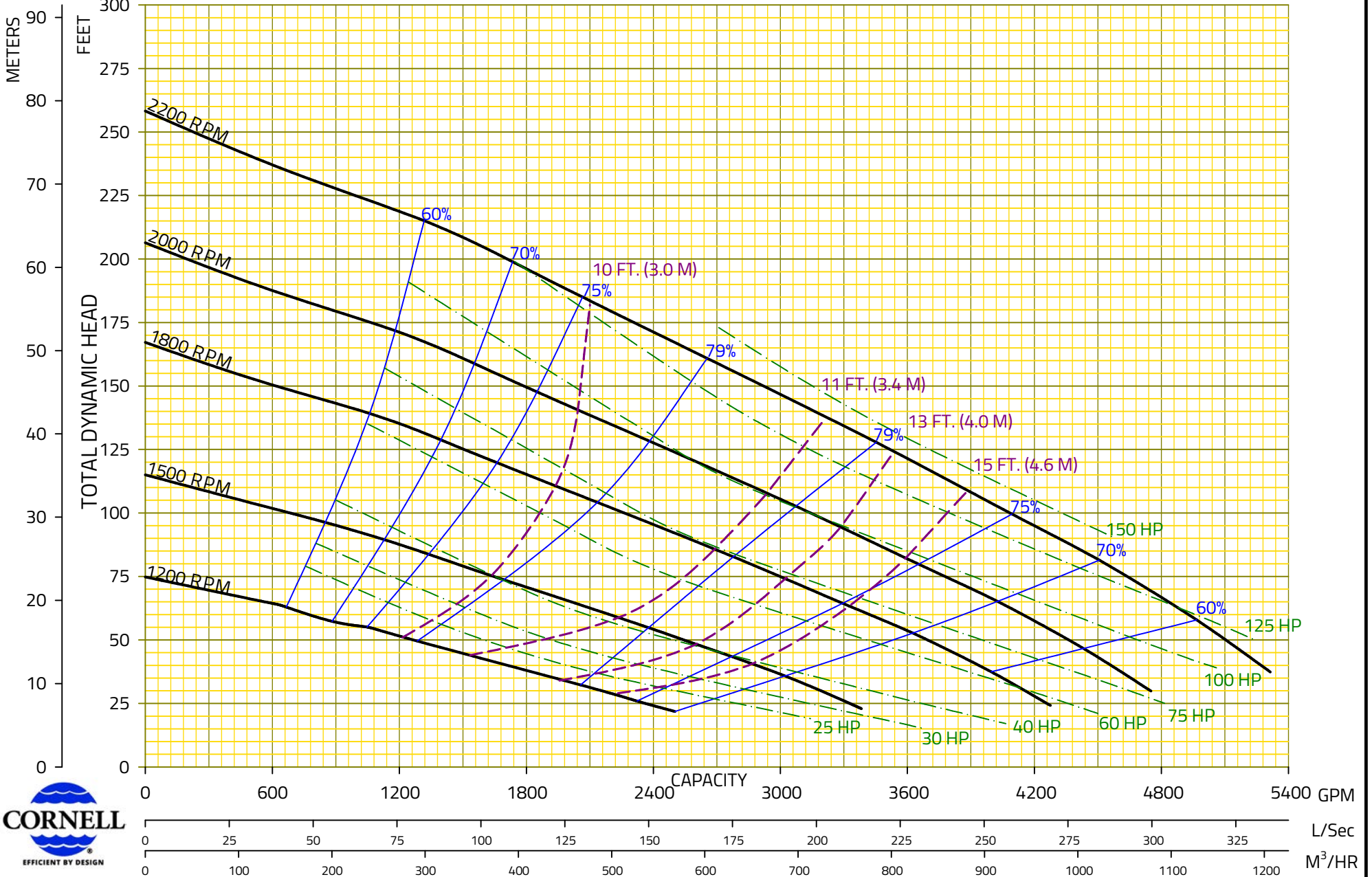
PROPOSAL CURVE, ACTUAL DATA MAY VARY +/- 10%
